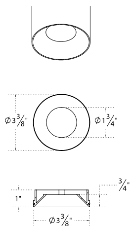
B3R-328-DC-TL
