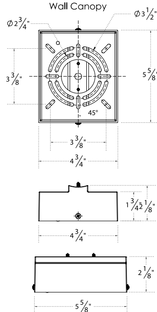
Wall Canopy
